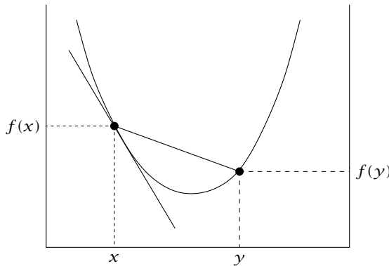
Figure A.7: A convex function.
