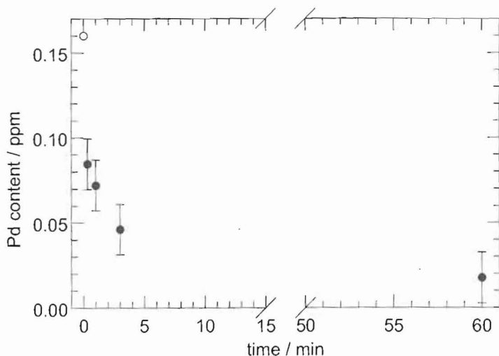
Figure 27.2. Analysis of soluble Pd from \text{BaCe}_{0.95}\text{Pd}_{0.05}\text{O}_{2.95} by ICP, as a function of reaction time (reagents and conditions: 3.0 mg \text{BaCe}_{0.95}\text{Pd}_{0.05}\text{O}_{2.95} (0.05 mmol Pd), 4 mmol \text{K}_2\text{CO}_3 , 1.0 mmol 4-bromoanisole, 1.5 mmol \text{PhB}(\text{OH})_2 , 12 mL IPA- \text{H}_2\text{O} (1:1, v/v), 80^\circ\text{C} ). The measurement for t = 0 min corresponds to the catalyst stirred with \text{K}_2\text{CO}_3 in IPA/ \text{H}_2\text{O} (i.e., in the absence of the aryl halide) at 80^\circ\text{C} for 1 h.
