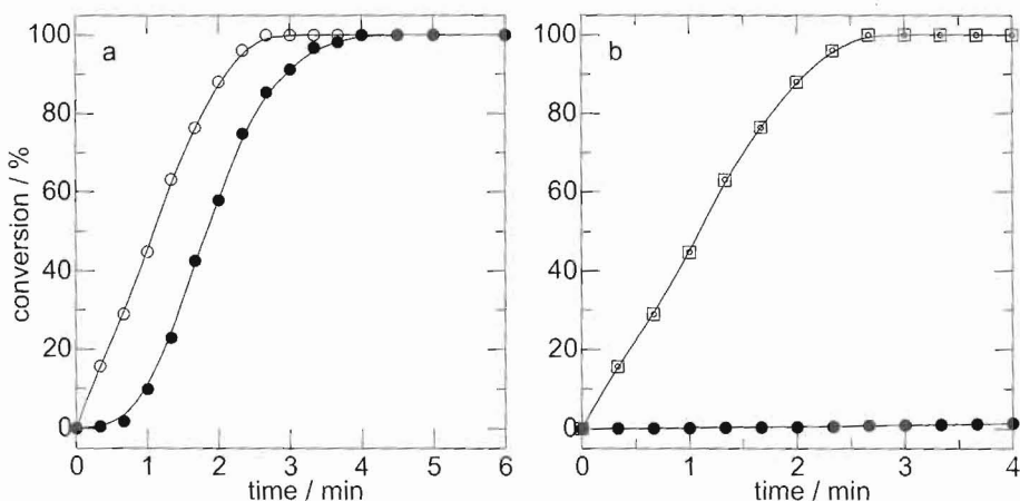
Figure 27.1. Kinetic profiles for the coupling of 4-bromoanisole with phenylboronic acid to yield 4-bromonaphthalene, (a) using as-prepared \text{BaCe}_{0.95}\text{Pd}_{0.05}\text{O}_{2.95} (open circles) or \text{BaCe}_{0.90}\text{Pd}_{0.10}\text{O}_{2.90} (filled circles) as the catalyst; and (b) using \text{BaCe}_{0.95}\text{Pd}_{0.05}\text{O}_{2.95} as-prepared (small open circles); reduced (filled circles); and reoxidized (open squares) as the catalyst. Reagents and conditions: 3.0 mg catalyst (0.05 mol % Pd, x = 0.05 ; 0.10 mol % Pd, x = 0.10 ), 1.0 mmol 4-bromoanisole, 1.5 mmol \text{PhB}(\text{OH})_2 , 4.0 mmol \text{K}_2\text{CO}_3 , 12 mL IPA- \text{H}_2\text{O} (1:1, v/v), 80°C. Lines are drawn only to guide the eye.
