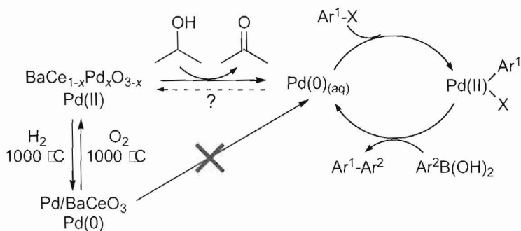
Scheme 27.1. Proposed mechanism for Suzuki coupling by Pd-doped perovskite catalysts.
