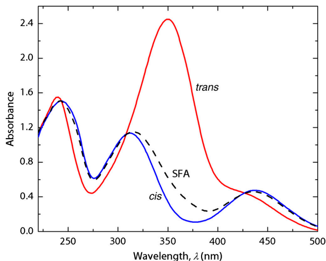
Fig. S1. UV-visible spectrum for 0.2 mM trans and cis azoTAB (red and blue solid curves, respectively), and for 0.2 mM azoTAB equilibrated in the SFA (white light) illumination with UV light shining through the front window of the SFA chamber (black dashed curve). This result confirms that during force measurements of cis azoTAB monolayers and layers, the amount of trans azoTAB present in the layers was negligible.
