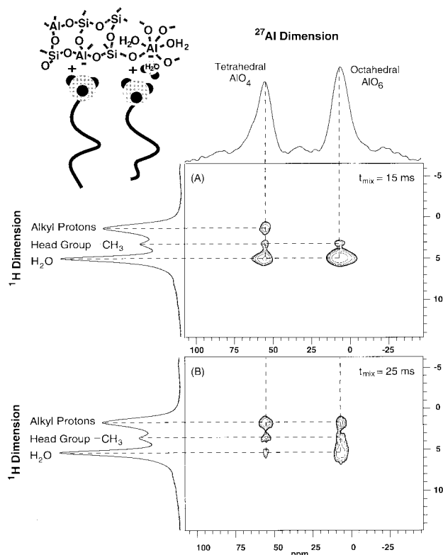
Figure 9. 2D ^{27}\text{Al}\{^1\text{H}\} HETCOR spectra for the same hydrothermally synthesized aluminosilicate MCM-41h sample used in Figure 8 but acquired using the pulse sequence in Figure 1b, which allows for ^1\text{H} spin diffusion to occur during an added mixing time. (a) For a mixing time of 15 ms, intensity correlations are observed between tetrahedral ^{27}\text{Al} sites and protons associated with ammonium methyl groups, alkyl CTA ^+ chains, and adsorbed water and between octahedral ^{27}\text{Al} sites and protons associated with ammonium methyl groups and adsorbed water. (b) A longer mixing time of 25 ms leads to the appearance of additional correlated intensity between octahedral ^{27}\text{Al} species and the alkyl protons of the CTA ^+ surfactant chains. Aside from the insertion of the additional pulse and mixing time, the experimental conditions for this experiment were identical to those presented in Figure 8. Use of a very short mixing time, e.g., ( t_{\text{mix}} = 1 ms), yields a ^1\text{H} spin diffusion HETCOR spectrum (not shown here) that is identical to the one in Figure 8, as expected for the limiting case of negligible ^1\text{H} spin diffusion.
